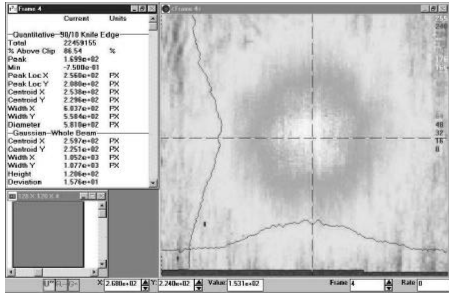
Fig. 8 - Transversal intensity profile of the laser beam (2D) -.
