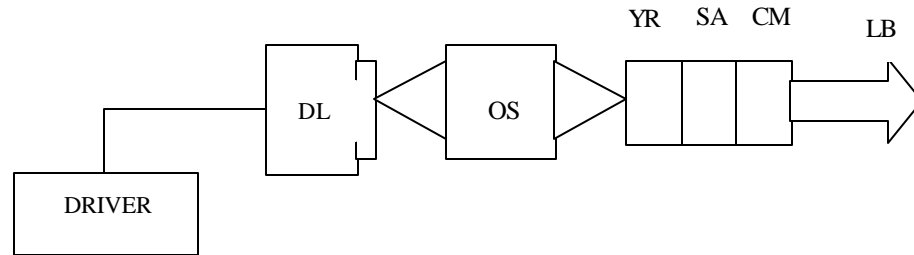
Fig.1 - Schematic set-up of the microlaser; DL : pump diode laser; OS : collimation/focusing optical system; YR : Nd:YAG rod ; SA : saturable absorber; CM : coupling mirror; LB : laser beam-
