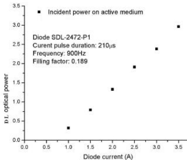
Fig. 5. - The pump system efficiency characteristic for SDL 2472-P1 laser –.
