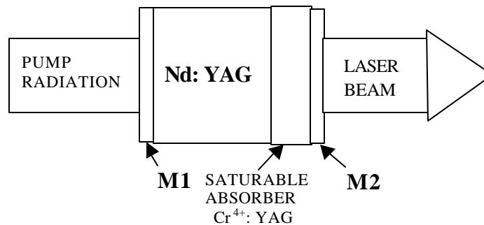
Fig.3 - Microchip laser resonator. Nd: YAG: laser active medium; M1: dichroic laser mirror (HR at 1064 nm, HT at 808 nm); M 2: laser mirror partial reflective at 1064 nm -.
