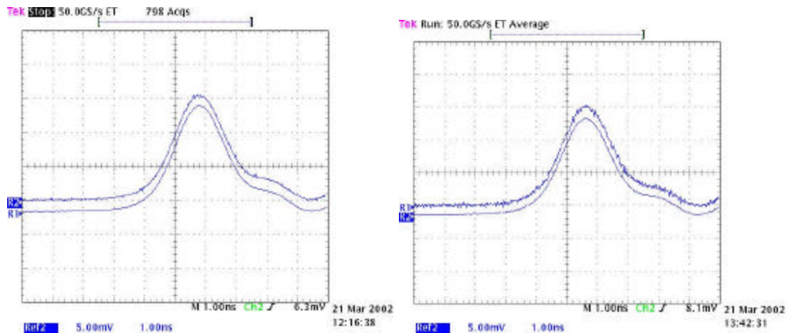
Fig. 10. -The time evolution of the laser pulse temporal profile -.
