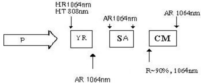
Fig.2 - Laser resonator with discrete optical components. YR : active medium Nd: YAG; SA : saturable absorber Cr: YAG; CM : coupling mirror; P : pump beam; HR : high-reflectivity dielectric coating; AR : antireflective dielectric coating -.
