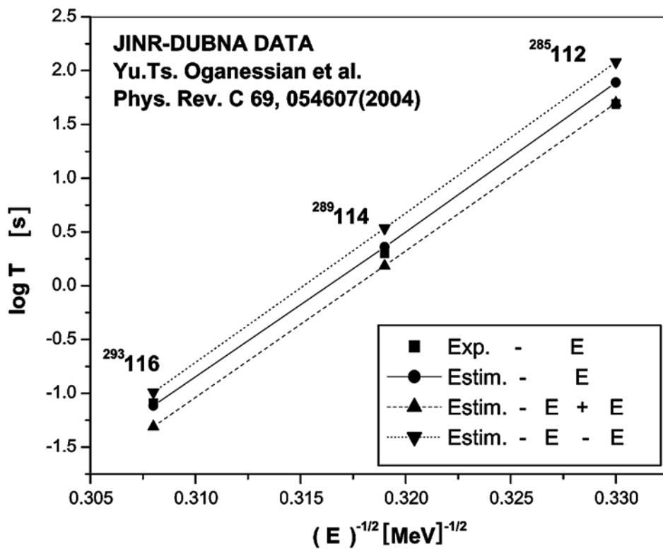
Fig. 6 – Same as in Fig. 3, but for 293 116.
