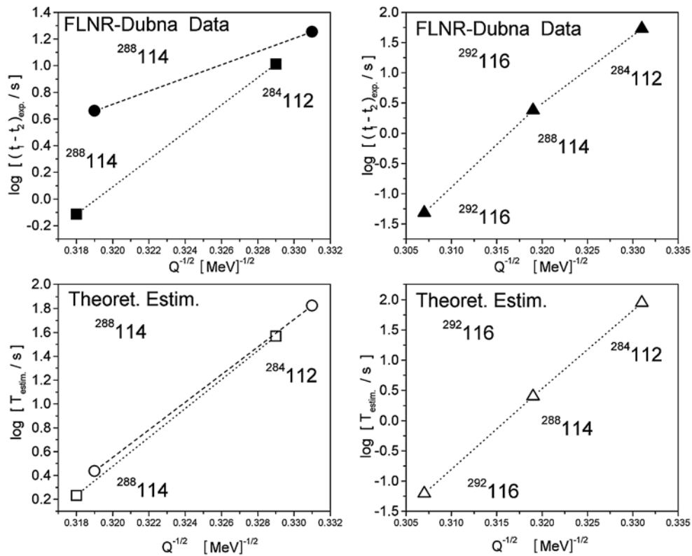
Fig. 2 – Summary of the \alpha -decay data obtained by Oganessian et al. [40–42] for ^{287-289}_{114} isotopes and estimated \alpha -half-lives.
