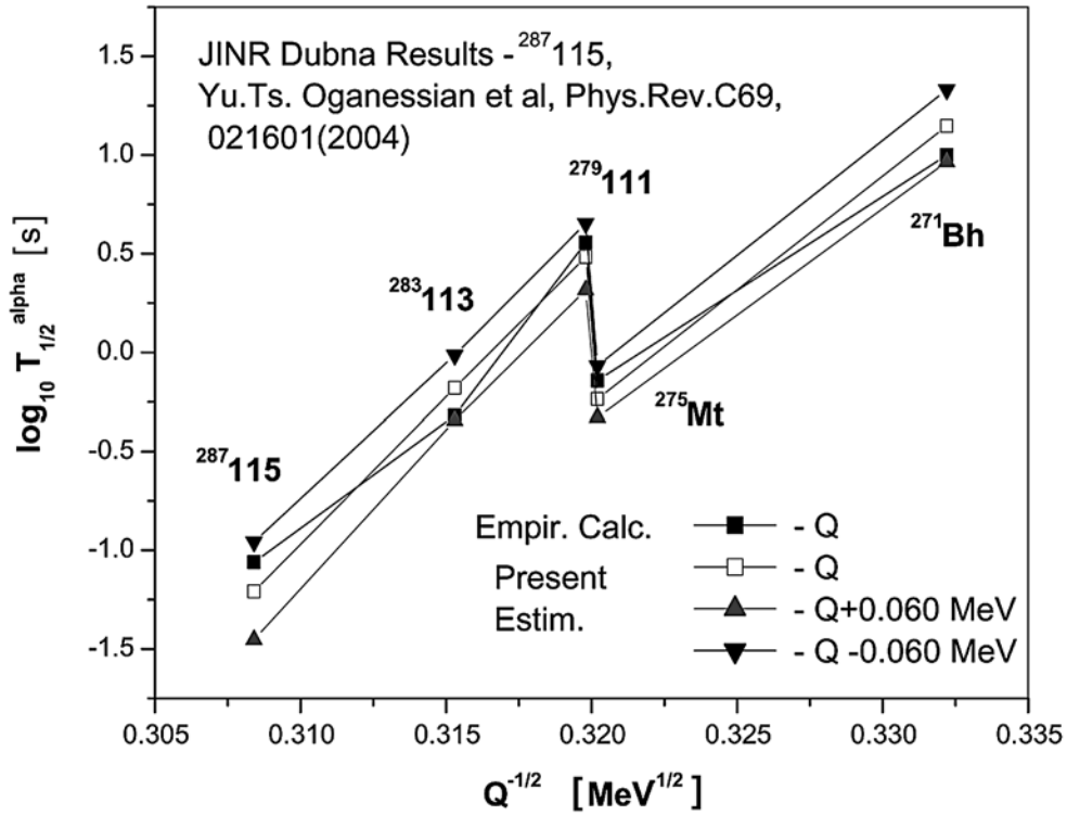
Fig. 3 – The Gamow plot for experimental [44] and estimated \alpha -half-lives for the decay chain of ^{287}115 .
