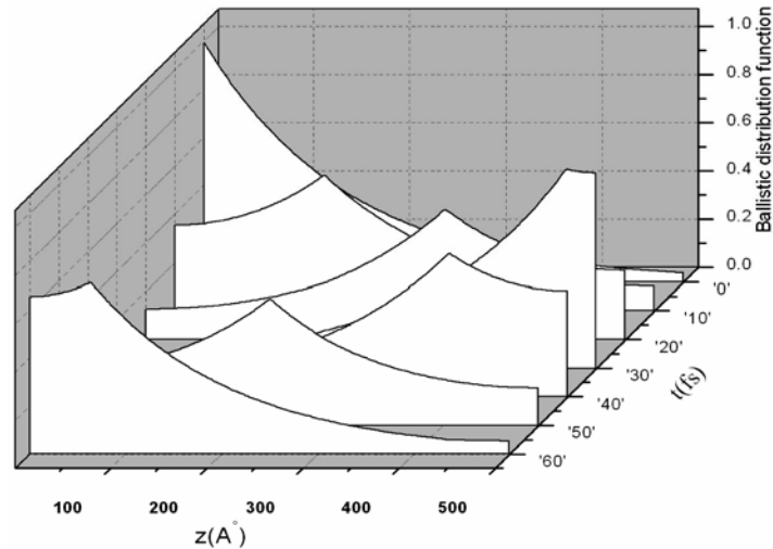
Fig. 1 – Ballistic distribution function at different times after the application of the \delta laser pulse calculated for a gold film of 500 \text{\AA} and an electron energy E = E_f + 1.4 eV.
