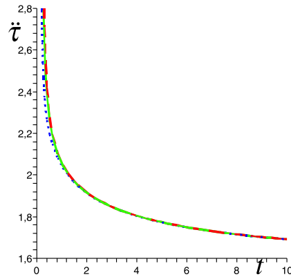
Fig. 3 – Acceleration of the Universe corresponding to a positive \lambda .
