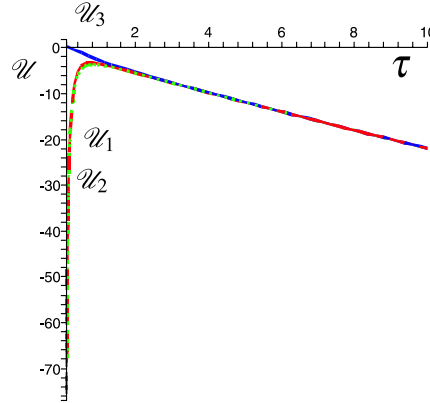
Fig. 2 – View of the potential \mathcal{U}(\tau) for \lambda > 0 .
