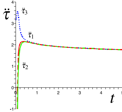
Fig. 4 – Acceleration of the Universe in case of a negative \lambda .
