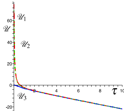
Fig. 1 – View of the potential \mathcal{U}(\tau) for \lambda > 0 .
