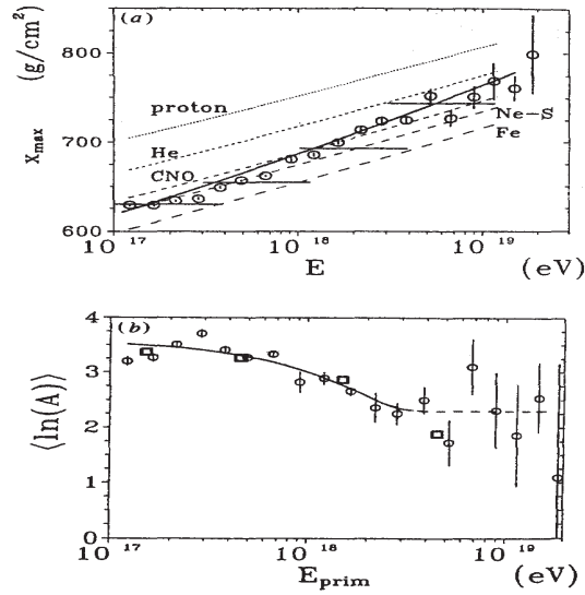
Fig. 4 – a) Depth of maximum ( X_{max} ) versus primary energy, E_{prim} . The lines are from ‘our’ calculations (1) and the points are from the Fly’s Eye experiment (Bird et al. , 1993); b) \langle \ln(A) \rangle versus E derived from (a) by linear interpolation. The curve is simply to guide the eye (from Wibig and Wolfendale, 1999).
