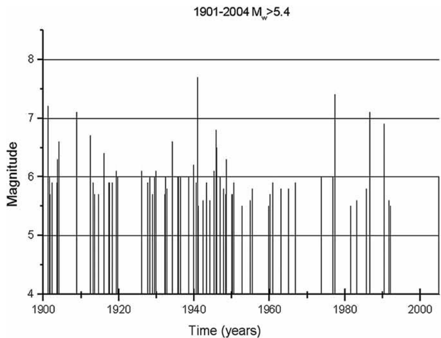
Fig. 5 – Seismic events of magnitude M_w > 5.4 recorded in the 1901–2004 time period [15].
