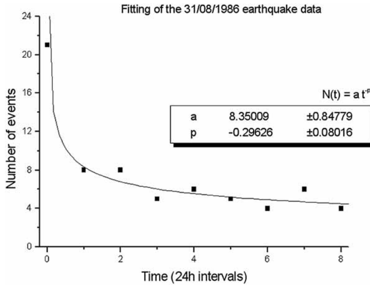
Fig. 9 – Fitting of the 31/08/1986 earthquake data (using [15]).
