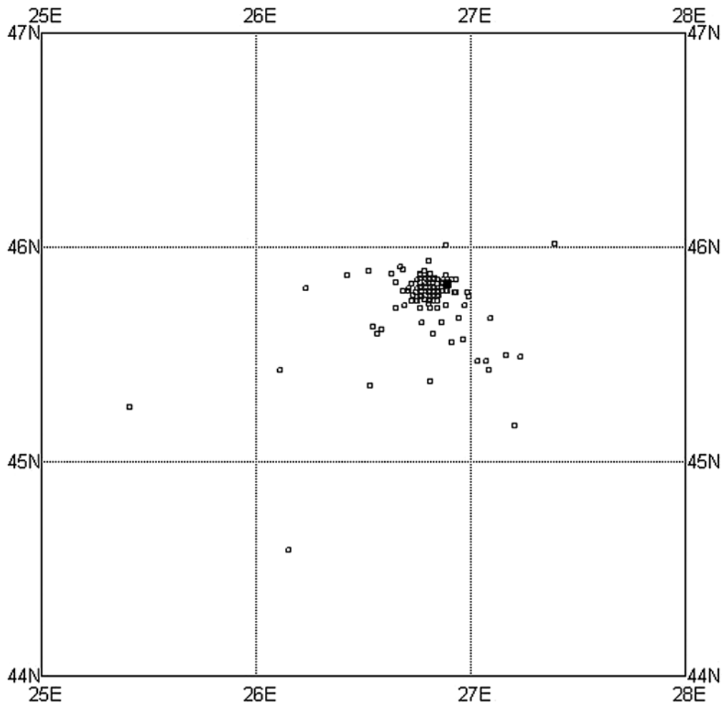
Fig. 11 – Latitude and Longitude of epicenters in the 30/05/1990–08/06/1990 time period [15].
