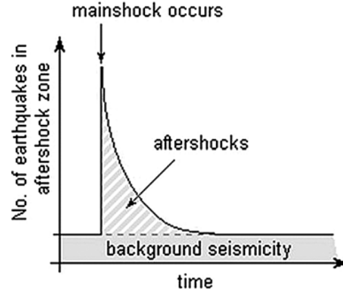
Fig. 6 – Decay of the seismic frequency after the main shock [23].
