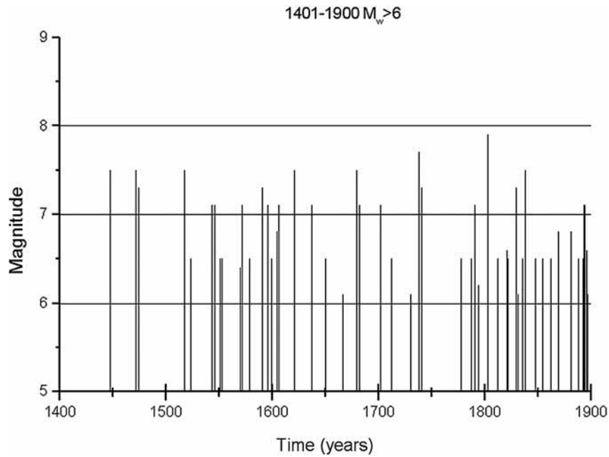
Fig. 4 – Seismic events of magnitude M_w > 6 recorded in the 1401–1900 time period [15].
