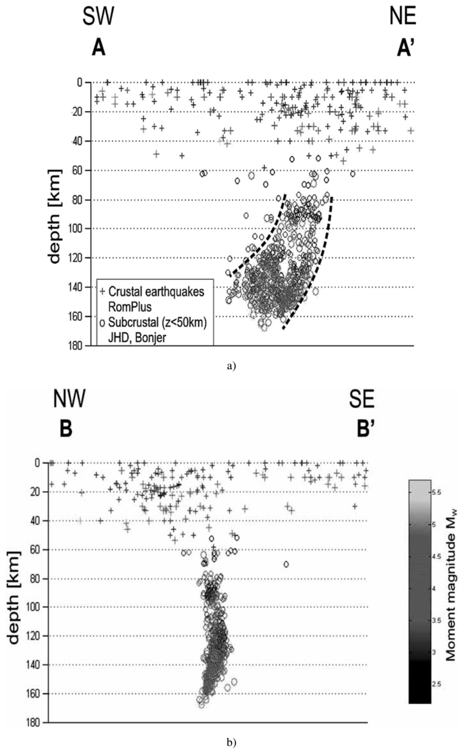
Fig. 3 – Hypocenters distribution on the NW-SE and NE-SW sections in the Vrancea area [8].
