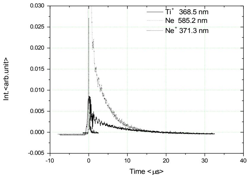
Fig. 2 - The emission profile of Ne, Ne + and Ti + spectral lines.
