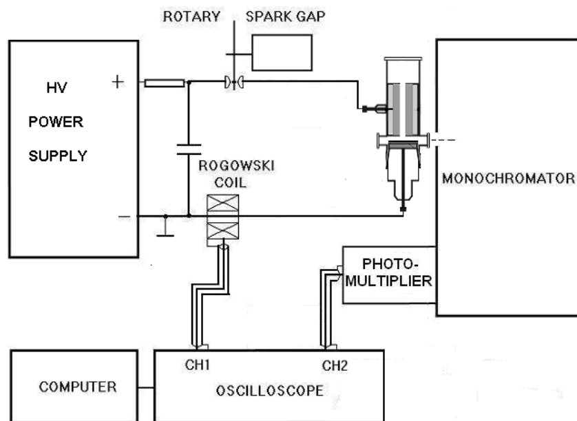
Fig.1 - Experimental setup.
