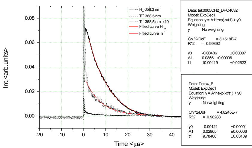
Fig. 3 - The emission lines of Ti + and H α and the corresponding fitting curves.
