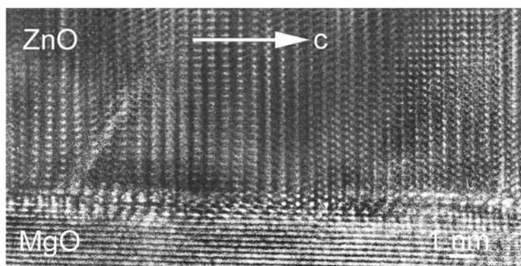
Fig. 7 – High resolution TEM in cross section of the interface between the a axis oriented ZnO layer grown on MgO single crystal.
