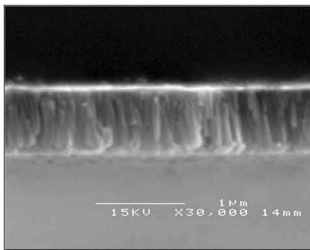
Fig. 4 – Scanning electron microscopy images in cross section of a layers prepared in the following experimental conditions: \lambda = 1060 nm, laser fluence 20 \text{ J/cm}^2 , oxygen pressure 0.05 \text{ mbar} , substrate temperature 350^{\circ}\text{C} , Pt coated Si substrate.
