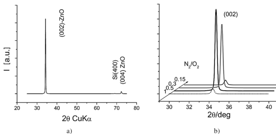
Fig. 9 – Representative XRD pattern of a nitrogen-doped ZnO film (N 2 /O 2 = 0.3 in the gas mixture) (a) and (002) peak at various concentrations of nitrogen in the gas mixture (b).
