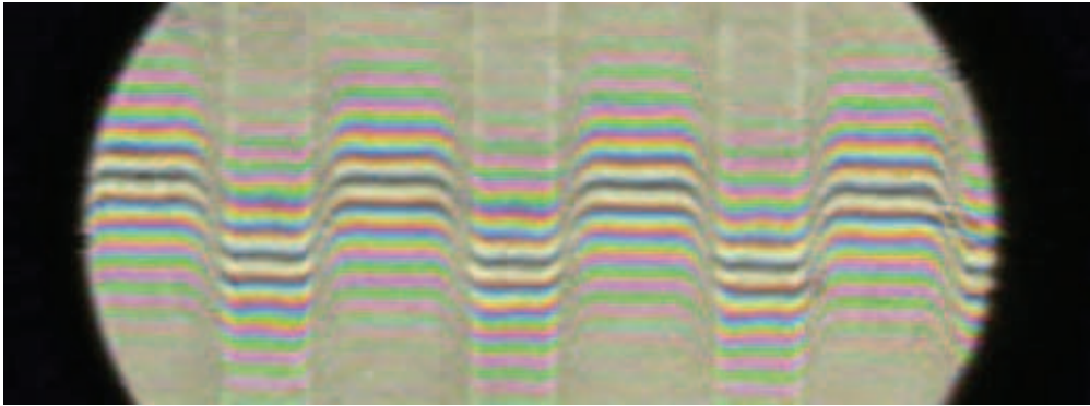
Fig. 4 – White and monochromatic fringes allow for the measurement of the integer and fractional part respectively of the number of \lambda/2 units of the height.
