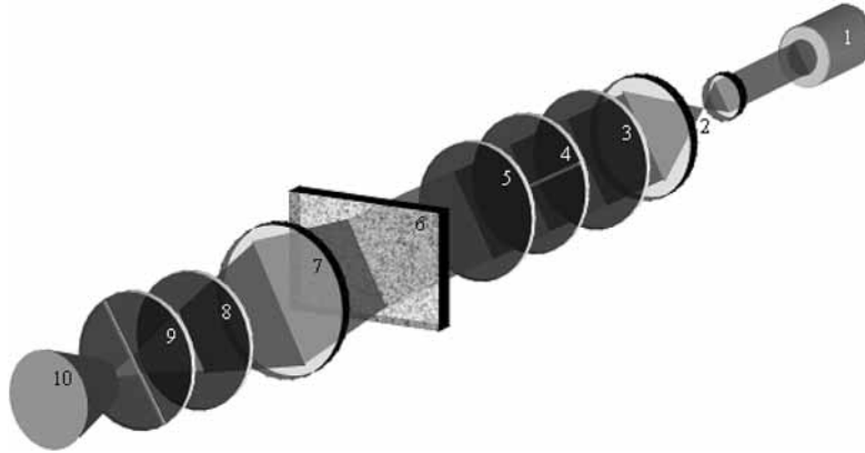
Fig. 2 – Optical scheme of the Mueller polarization imaging system.
