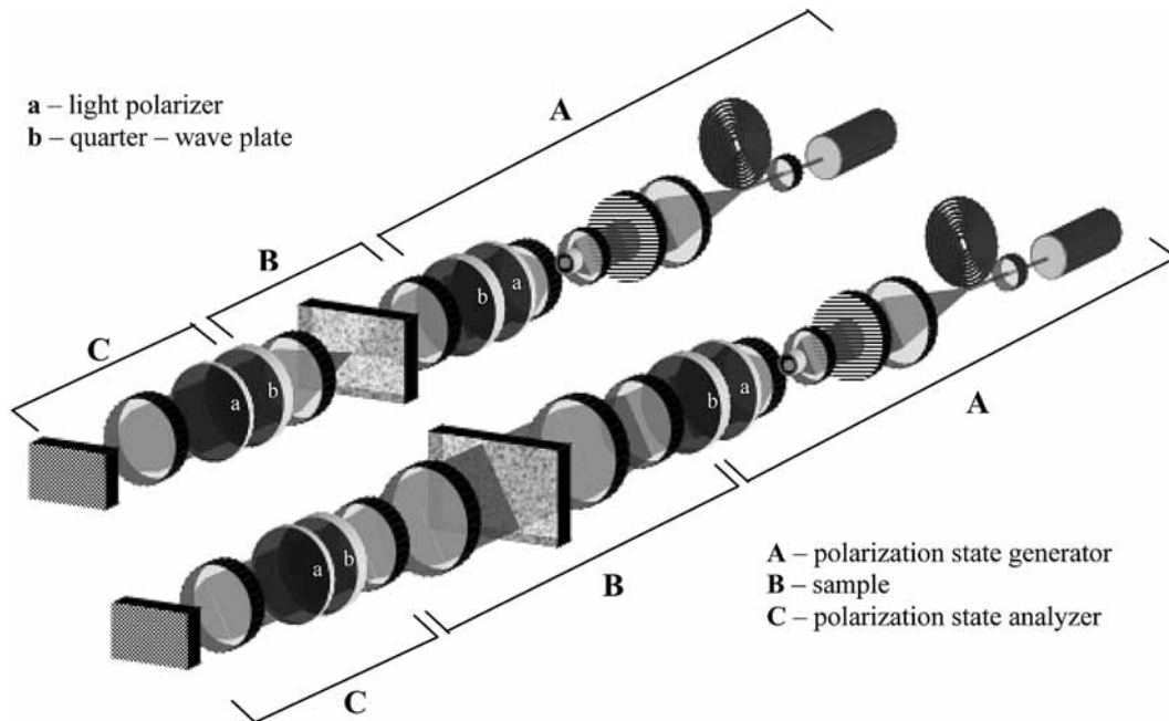
Fig. 1 – Classical configurations for a Mueller matrix imaging polarimeter, in the focused beam (above) or expanded beam (below) setup: a) light polarizer; b) quarter – wave plate.
