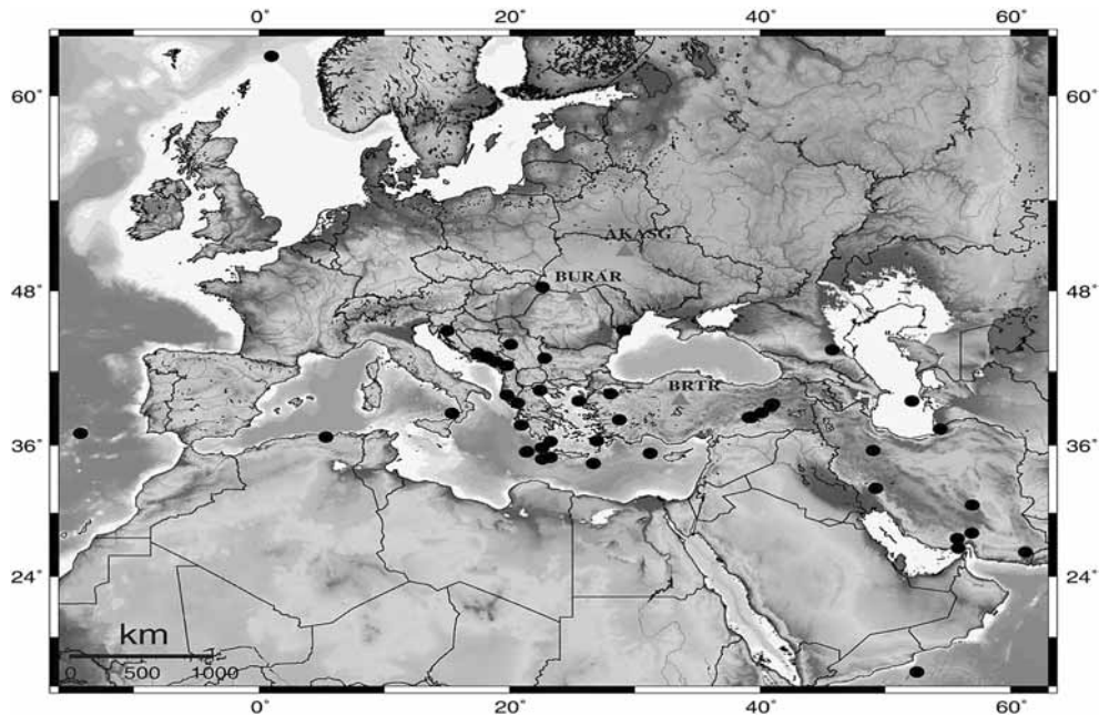
Fig. 2 – The epicentral map. Black dots are epicenters of data base events recorded between 2004 and 2007; BURAR, AKASG and BRTR arrays are represented by gray triangles.
