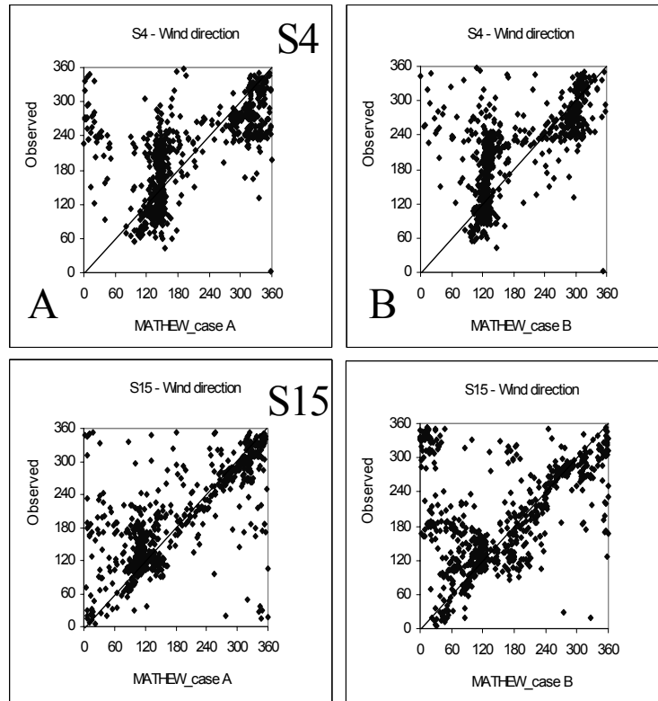
Fig. 2 – Scatter plots of the wind direction (degrees) modelled with MATHEW in case A, case B and the observations. The wind direction is measured at 10 m above ground, while the modelled wind direction corresponds to the middle of the first model layer (20 m thickness).
