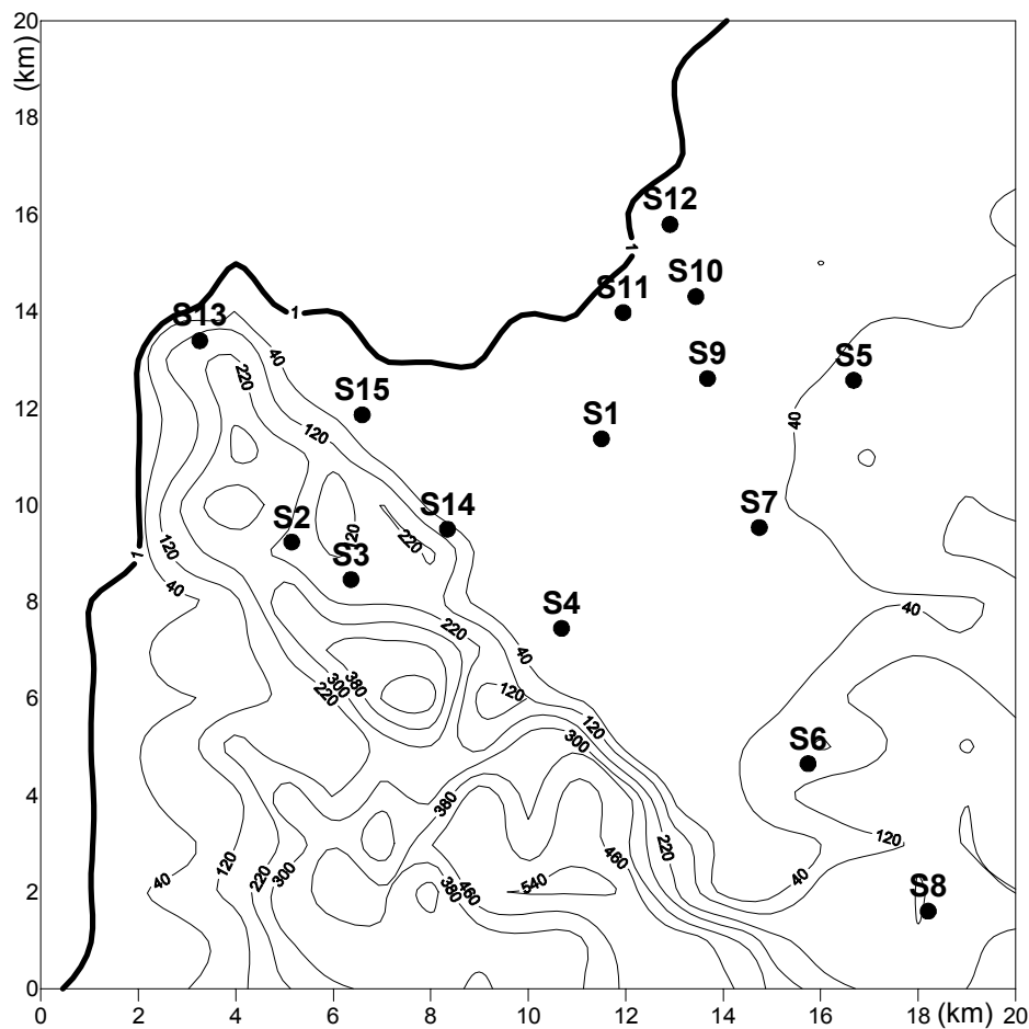
Fig. 1 – Modelling area showing land/sea and topography. Also included are the available meteorological sites.
