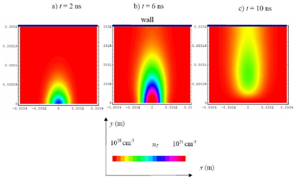
Fig. 3 – The contour curves of total atom density for various time moments as resulted from the numerical simulation of the diffusion equation in the presence of a wall.
