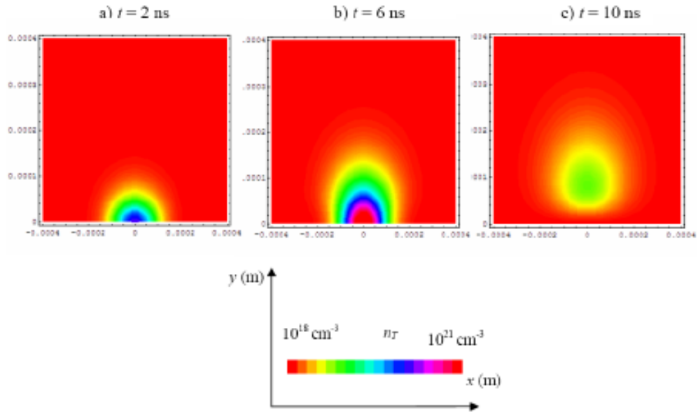
Fig. 2 – The contour curves of total atom density for various time moments as resulted from the numerical simulation of the diffusion equation.
