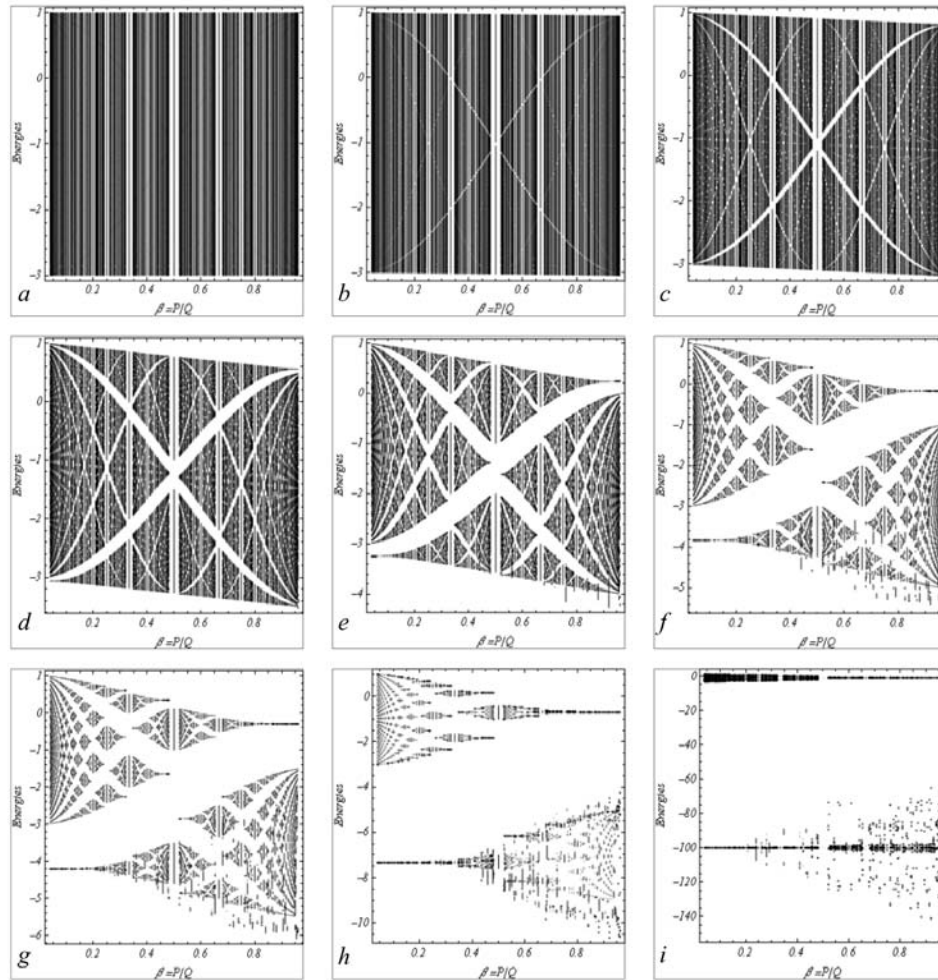
Fig. 1 – The energy spectrum versus \beta showing the band splittings for several n -values.
