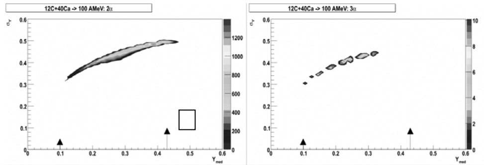
Fig. 2 – Mean rapidity deviation versus mean rapidity with FLUKA simulation code.
