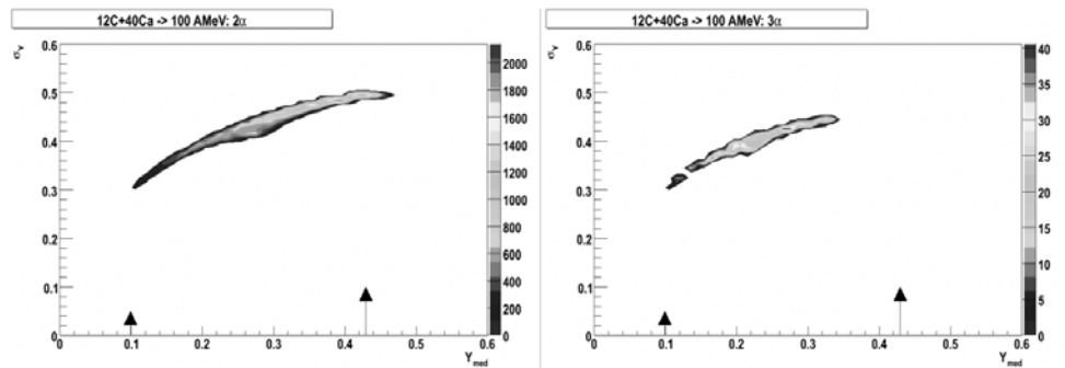
Fig. 3 – Mean rapidity deviation versus mean rapidity with Geant4-QGSP-BIC-HP simulation code.
