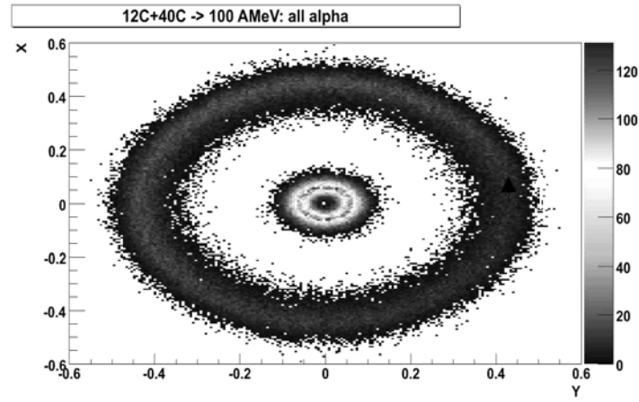
Fig. 1 – Simulation of nuclear sources emitting alpha particles with FLUKA.
