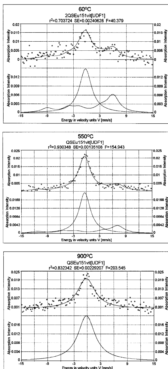
Fig. 4 – Some examples of fitted Mössbauer spectra.
