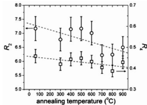
Fig. 2 – The ratios R_2, R_4 of the intensities of the electric- and magnetic-dipole transitions function of the annealing temperature. The dashed lines merely suggest the decrease of both R_2 and R_4 .
