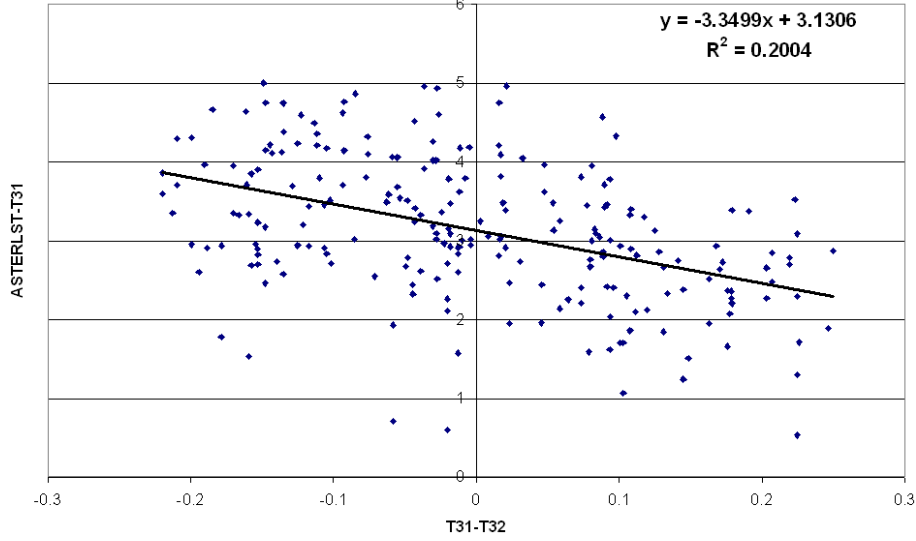
Fig. 1 – Graphic representation of (T_{\text{ASTER}} - T_{31}) and (T_{31} - T_{32}) differences.
