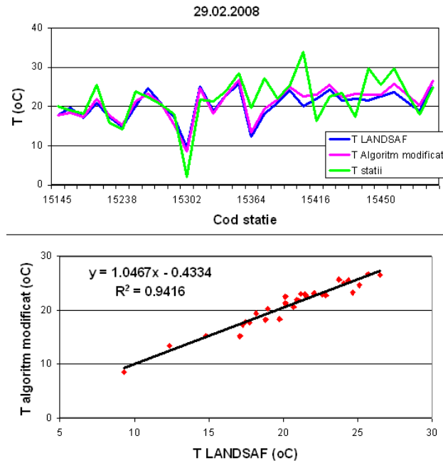
Fig. 4 – The graphic representation of the variation between T_{\text{algoritm}} , and T_{\text{LANDSAF}} on 29th of February 2008 (above) and the correlation relationship between them (below).
