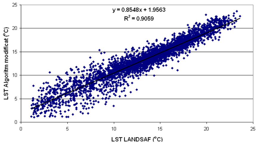
Fig. 5 – The graphic representation of the correlation between T_{\text{algoritm}} , and T_{\text{LANDSAF}} on 29th of February 2008.
