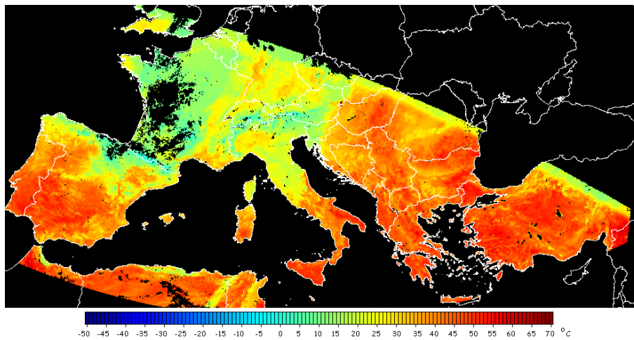
Fig. 2 – LST LANDSAF product covering Europe, from 23.08.2007.
