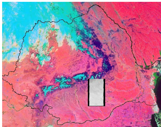
Fig. 3 – MODIS/TERRA image, colour composite ch3-ch2-ch1, from 04.04.2004 and the location of the two ASTER images.
