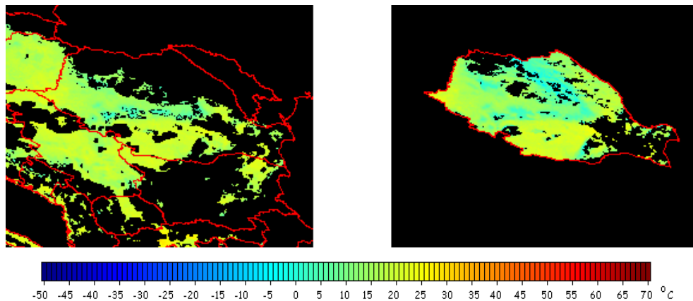
Fig. 6 – LST LANDSAF product (left) and LST adapted algorithm (right) for 28.02.2008, 13:30 GMT
