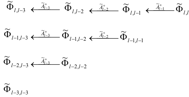
Fig. 1 – The functions \tilde{\Phi}_{l,m} .
