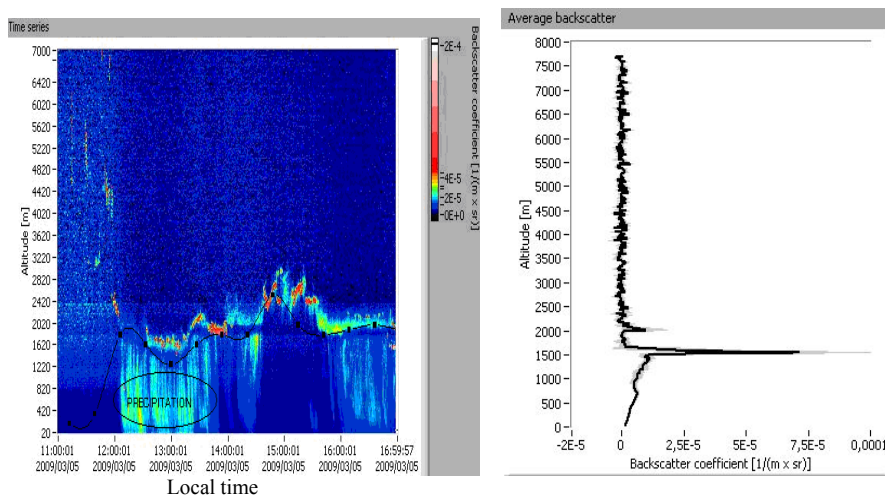
Fig. 1 – Image of the PBL (left) and associated backscatter profile (right) for 05 th of March 2009. The solid curve marks out the mixed layer height; the period with precipitation is also marked. The backscatter profile shows the mixed layer at the same height as in image (appropriate on 1500m).
