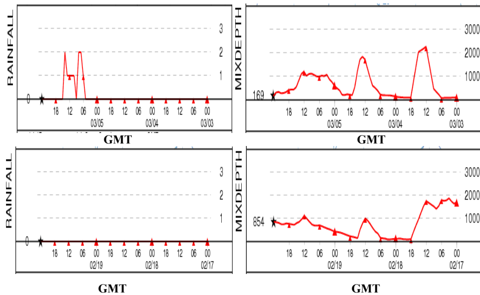
Fig. 3 – Meteorgrams obtained using HYSPLIT 4 [9]: precipitation left column and mixed layer height on right column; upper panel 05 th of March 2009 and lower for 19 th of February 2009.
