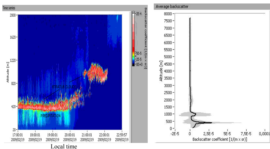
Fig. 2 – As in Fig. 1 but for 19 th of February 2009 in evening hours. In backscatter profile can be observed the two levels of the PBL marked by the cloud bases.
