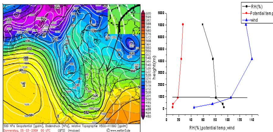
Fig. 4 – Synoptic map (left part, [10]) and vertical profiles of potential temperature, wind direction and relative humidity (right part) for 05 th of March 2009.
