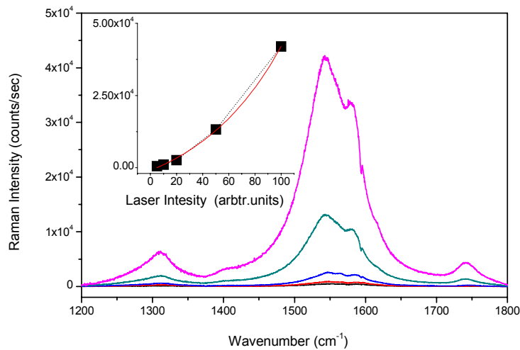
Fig. 7 – Stokes SERS spectra at resonant excitation \lambda_{exc} = 676.4 nm of SWNTs deposited as thin film on a diffraction grating covered with Au. In the inset reveals an exponential dependence on the intensity of the exciting light.
