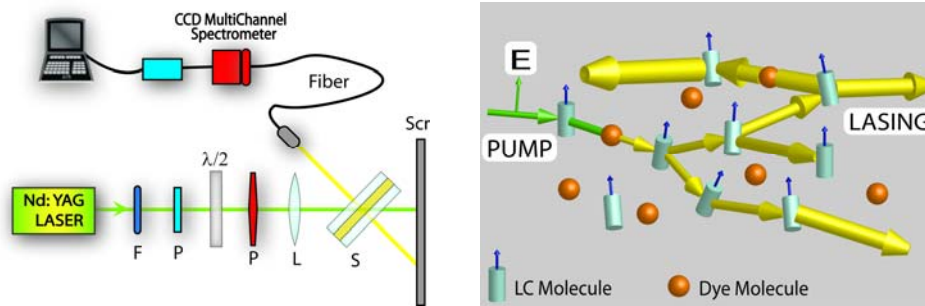
Fig. 1. – Schematic diagram of the experimental set-up (left): F is a filter, P – polarizers, \lambda/2 – wave plate, L – lens, S – sample, Scr – observation screen. Recurrent multiple light scattering in dye doped nematics provides the feedback for laser oscillations (right).
