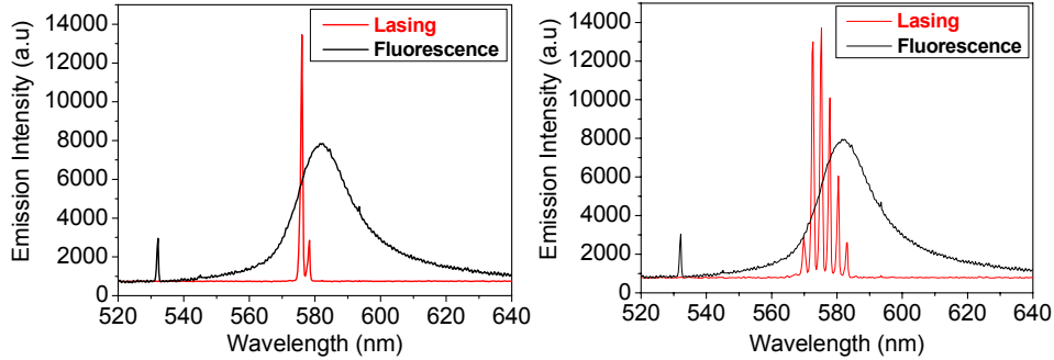
Fig. 3 – Fluorescence and random lasing spectra in the case of a sandwich cell upon increasing the pump energy. Discrete sharp peaks emerge from the residual spontaneous emission for pump energy density above 30\text{-}40 \mu\text{J}/\text{mm}^2 (a). At higher pump values multiple lasing peaks are generated (b). For clarity, the residual fluorescence signal was ten times magnified.
