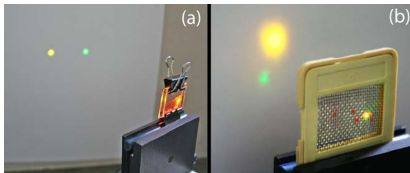
Fig. 2 – Different random lasing confinement geometries: a) sandwich cell; b) freely suspended film.
