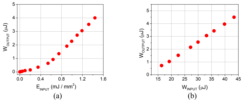
Fig.4 – a) Emission energy vs. pump energy density for the classic sandwich cell; b) output energy vs. input energy.
