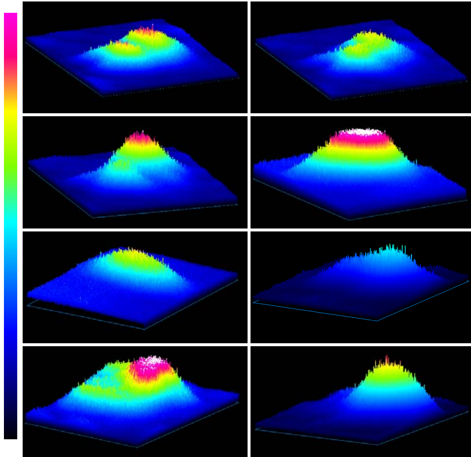
Fig. 5 – Spatial far field distribution of the intensities profile in a sandwiched ZLI 2659 doped sample for eight consecutive pump beam pulses illustrates a blinking behaviour in space and time.
