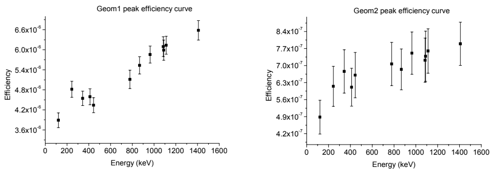
Fig. 2 – The peak efficiencies simulated with GEANT 3.21 for Geom1 (left panel) and Geom2 (right panel).
