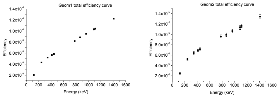
Fig. 3 – The total efficiencies simulated with GEANT 3.21 for Geom1 (left panel) and Geom2 (right panel).
