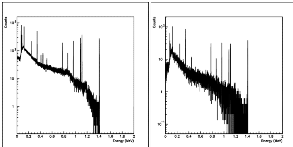
Fig. 1 – Spectrum simulated with GEANT 3.21 for a source of ^{152}\text{Eu} uniformly distributed in the waste drum; Geom 1 – left panel, Geom 2 – right panel.
